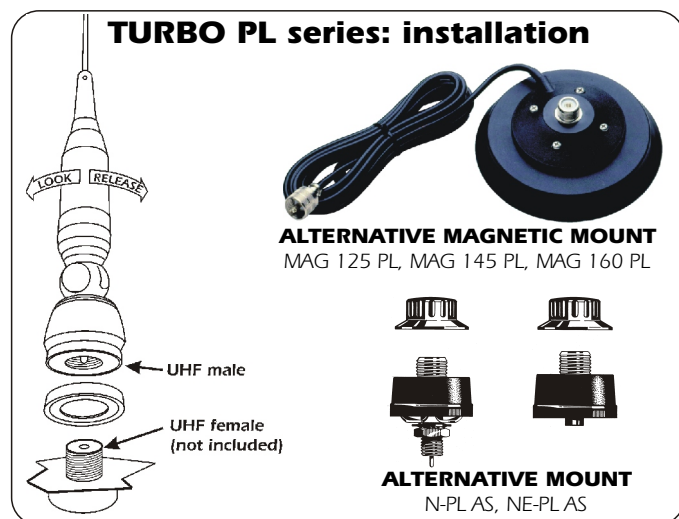
TURBO series: Hole installation
